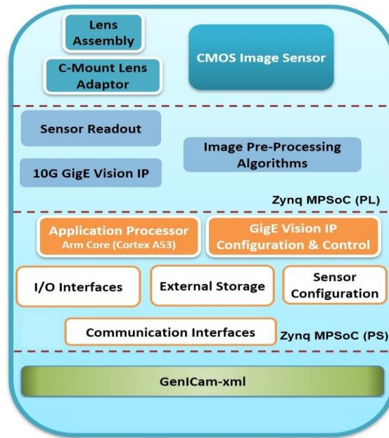
Fig. 1. iViS-10GigE architecture
